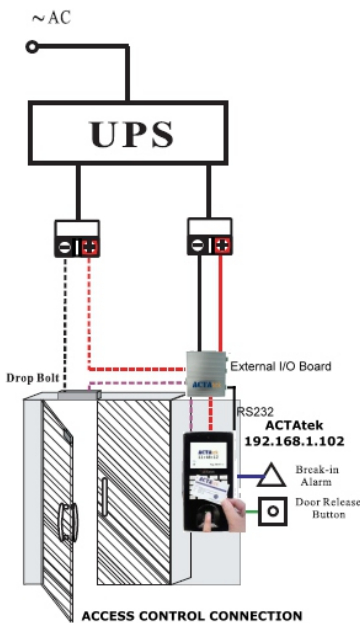
Figure: Connection diagram
