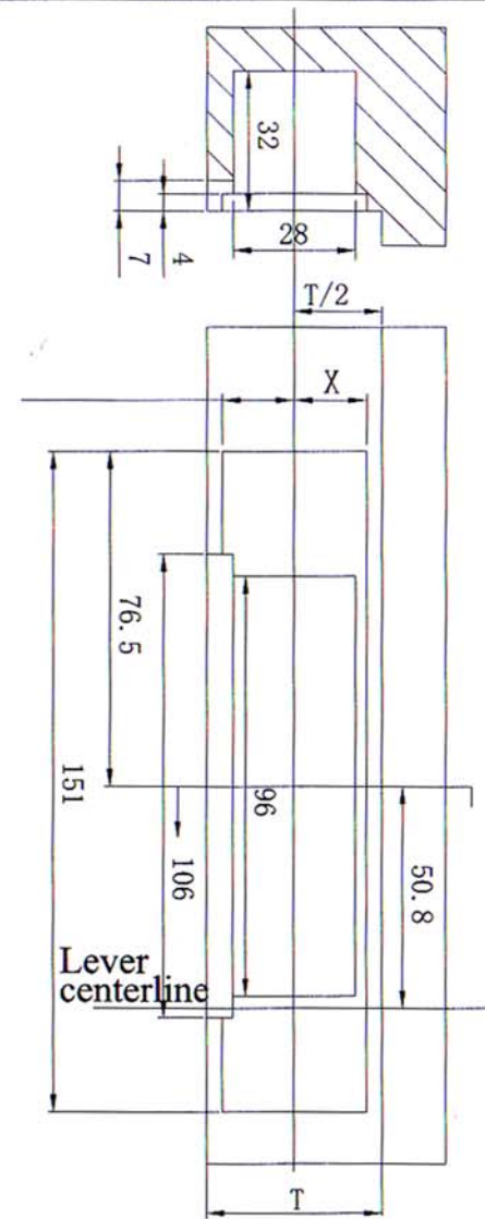
B. Drilling view of door frame
