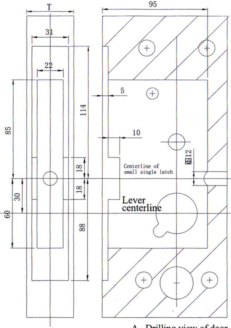
A. Drilling view of door
